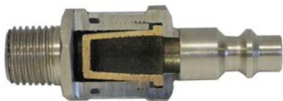
Sintered bronze element inside connector.
